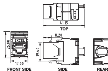
B. Keystone profiles. Dimensions in mm
